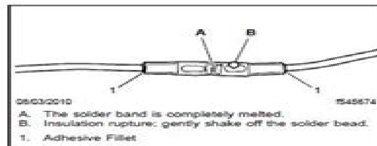
Fig. 4. Solder Bead Rupture
