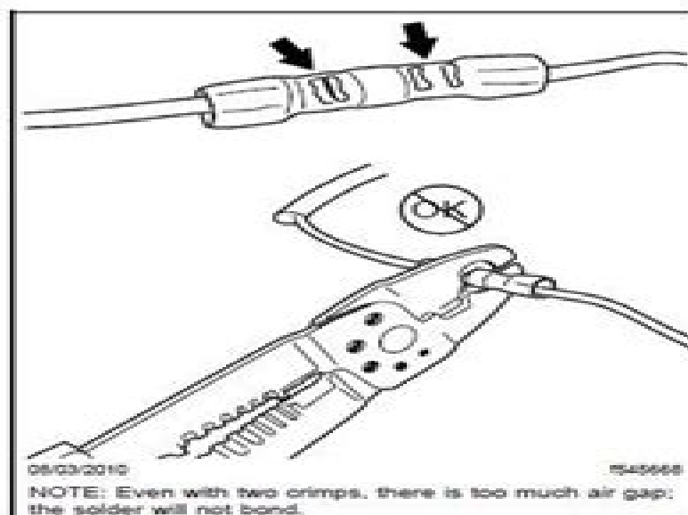
Fig. 3. Wrong Tool Being Used and a Crimp That Will Fail
